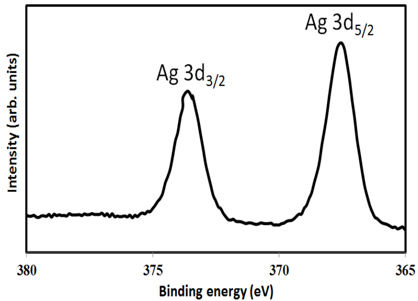
Figure 21 XPS spectra of the as-synthesized sample of Ag-ZnO nanowire
